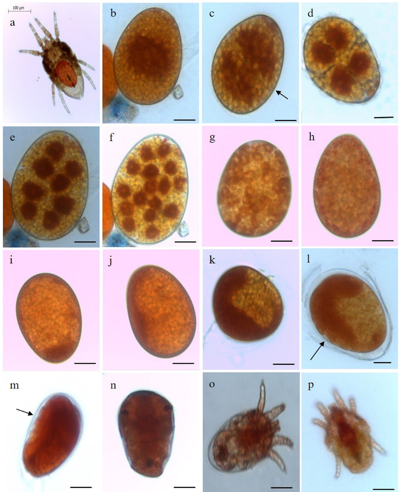
Figure 1 Development timeline of the Brevipalpus yothersi : (a) – B. yothersi female; (b) – Uncleaved egg: nucleus in the center of the egg; (c) – Two-cell stage embryo divided by visible membrane (arrow); (d) – Second cleavage; four-cell stage; (e) – Eight-cell stage; (f) – 16-cell stage; (g) – 128-cell stage; (h) – Migration of cells to the peripheral region: blastula formation; (i) – Visible germinal disc in the ventral region; (j) – Distension of the germinal disc on the side of the egg; (k) – Primitive body formation; (l) – Formation of metamers (arrow); (m) – Primordial appendages (arrow); (n) – Initiation of ocelli formation, more evident before (o) – hatching of the egg with emerging larva; (p) – Hexapod larvae seven days after oviposition. Scale bar length (a) 100 µm (magnification of 20x) and (b-p) 50 µm (magnification of 40x).
